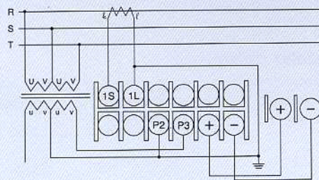
삼상삼선식 3Phase 3Wire Power Factor Meter Balance type
