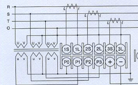
삼상사선식 3Phase 4Wire Power Factor Meter Unbalance type
