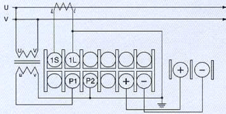
With Ext. Transducer (D-□□□□ Type)
