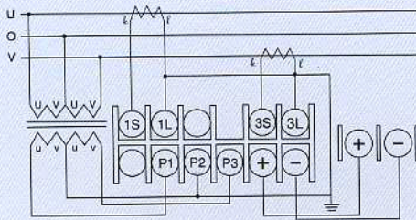
단상삼선식 1Phase 3Wire Power Factor Meter
