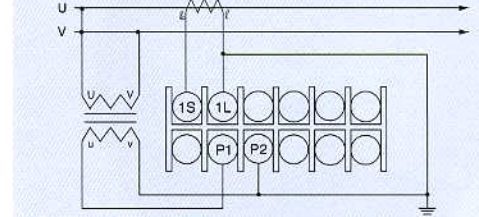
With Int. Transducer (D-□□□□T Type)
