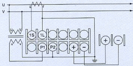
단상이선식 1Phase 2Wire Power Factor Meter
