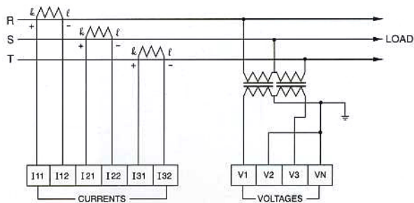
3상3선 V결선(2PT, 3CT) Mode No 3OP
