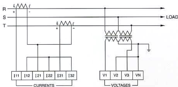
3상3선 V결선(2PT, 2CT) Mode No 3OP
