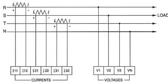
3상4선 Direct Y결선(3CT) Mode No 3P4L
