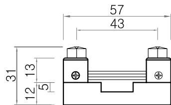
FRONT VIEW 1~50A(50~60mV)
