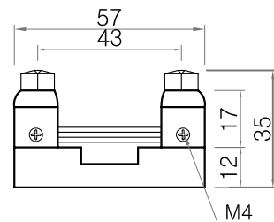
FRONT VIEW 60~90A(50~60mV)
